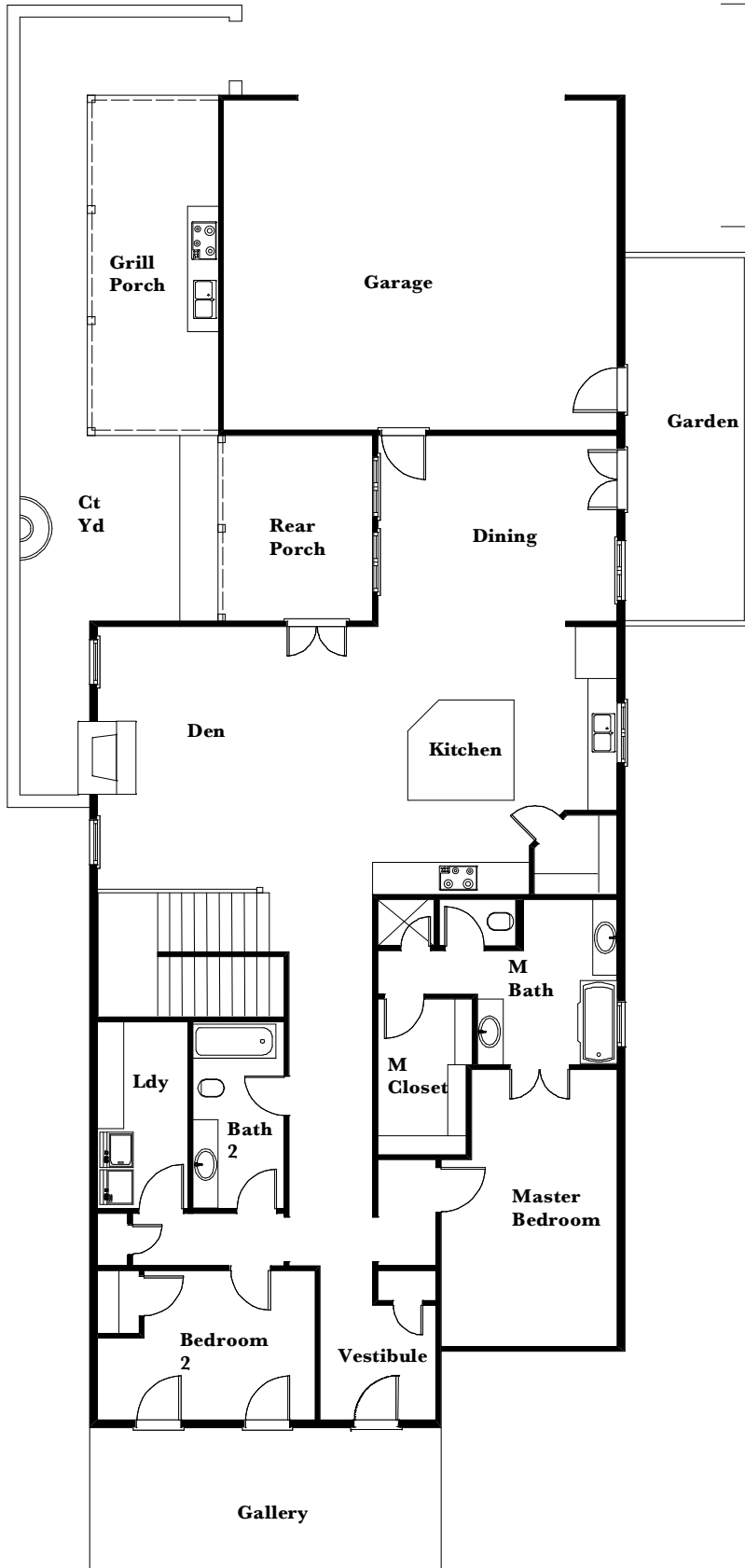
Carolina House Floor Plan
